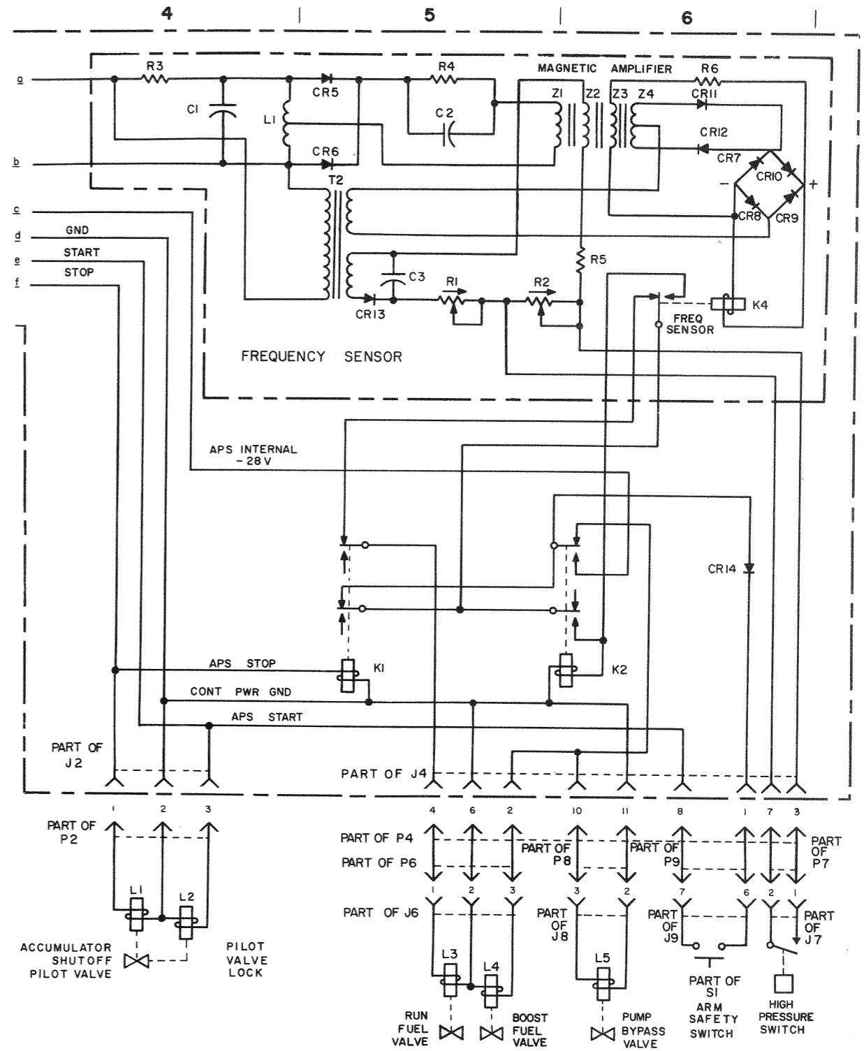
Figure 4-17 (U). Accessory power supply 9030900 electrical control system—functional schematic (serial numbers 69-3632 and subsequent) (sheet 2 of 2) (U).
