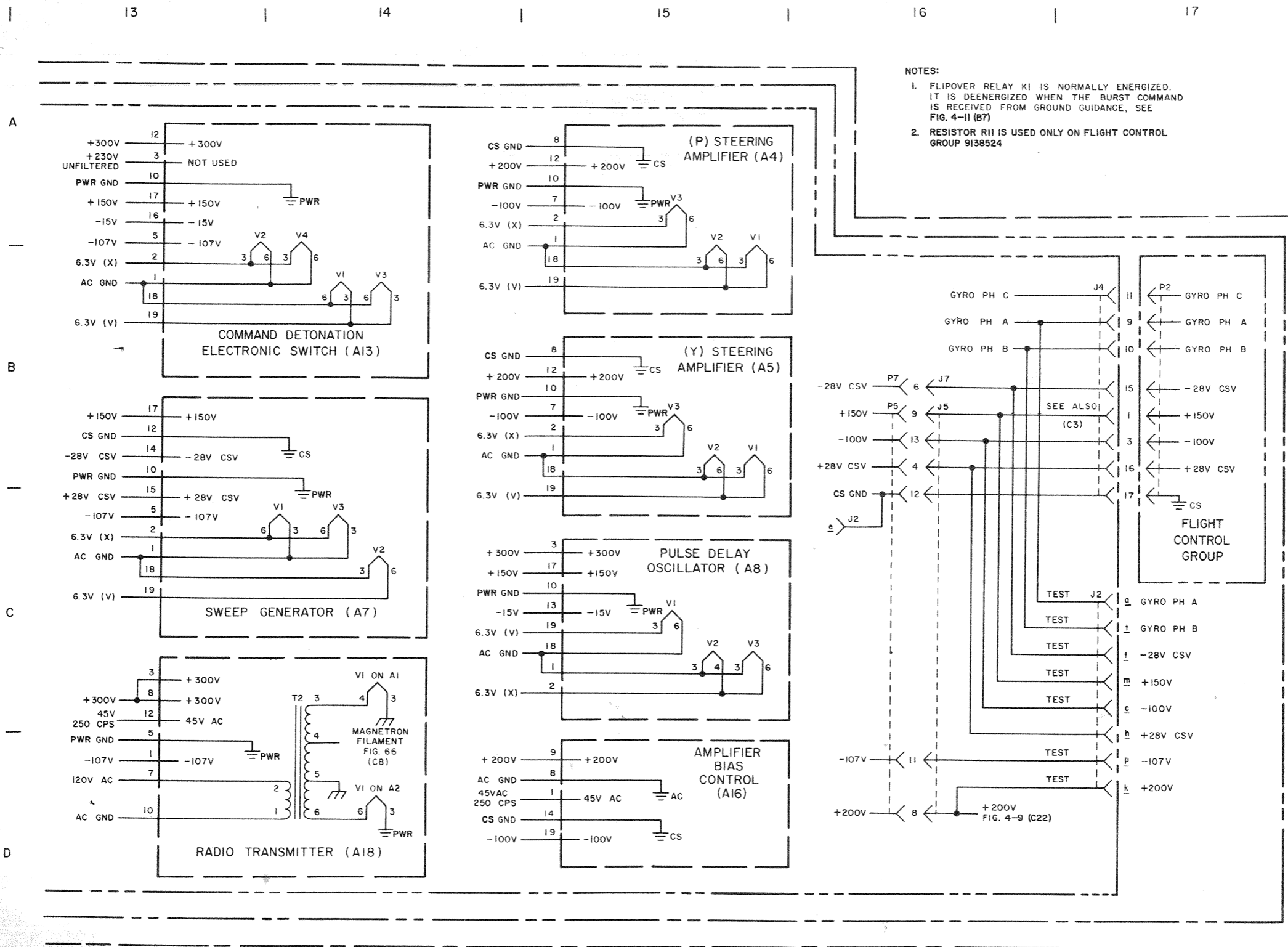
Figure 4-11 (C). Power supply and distribution circuit—functional diagram (mushroom) (sheet 3 of 3) (U).
