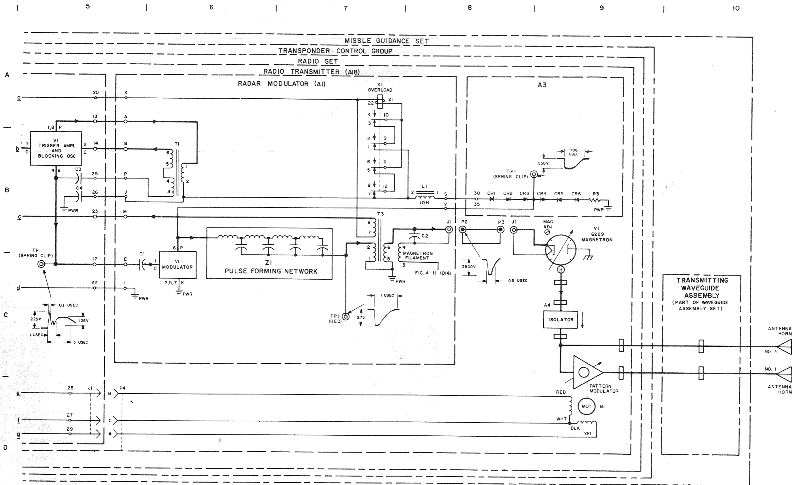
Figure 4-9 (C). Beacon transmitting circuit—functional diagram (mushroom) (sheet 2 of 2) (U).
