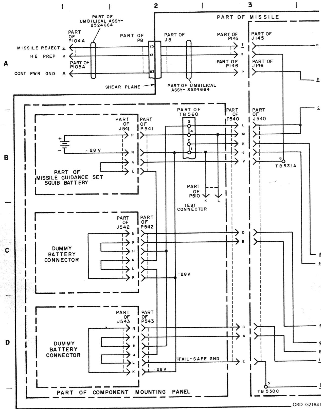
Figure 4-21 (U). Missile guidance set battery, missile reject, and HE prepared circuits—functional diagram (missiles 13684 and subsequent) (sheet 1 of 2) (U).
