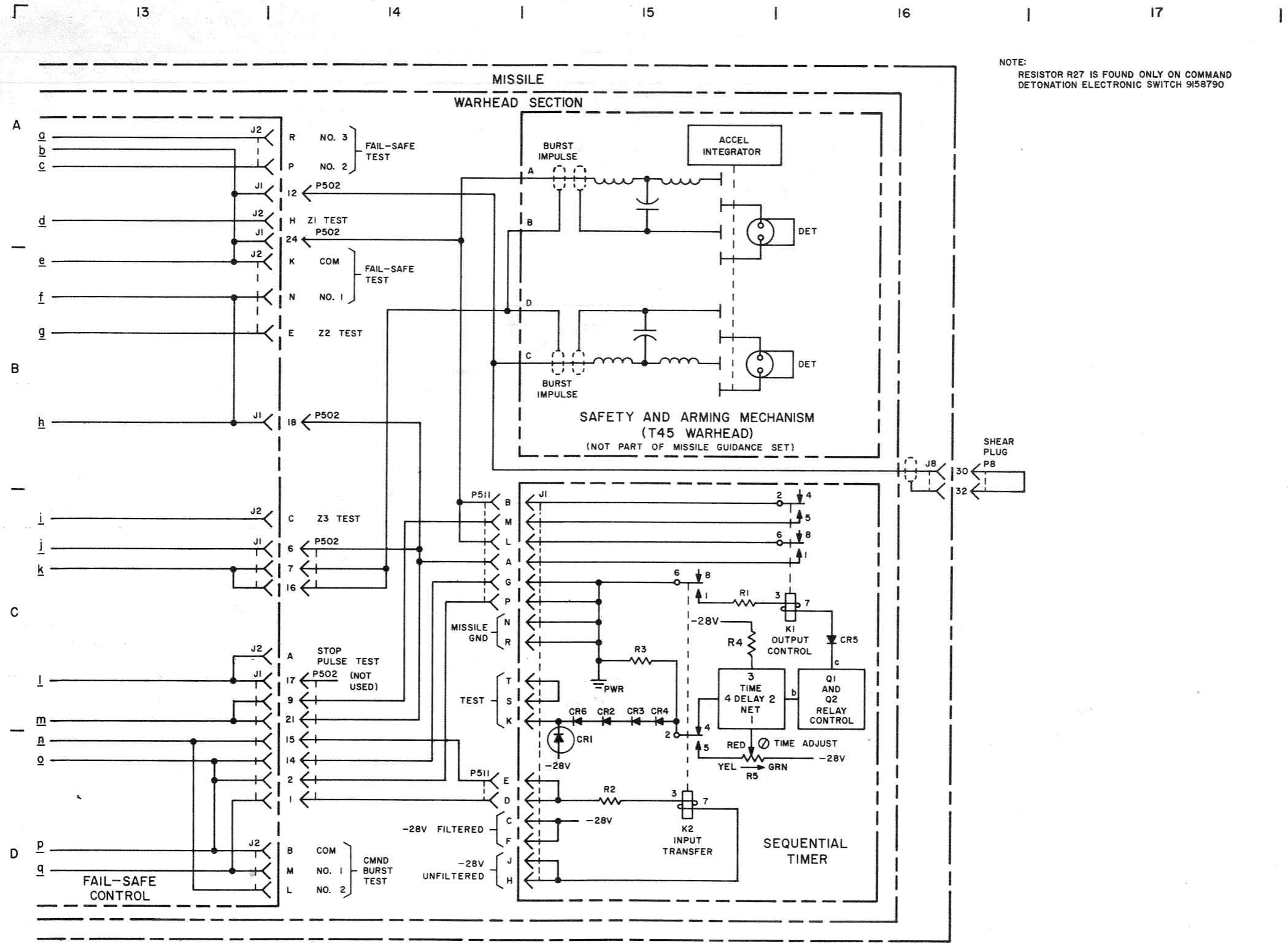
Figure 4-10 (C). Detonation command circuit—functional diagram (mushroom) (sheet 3 of 3) (U).
