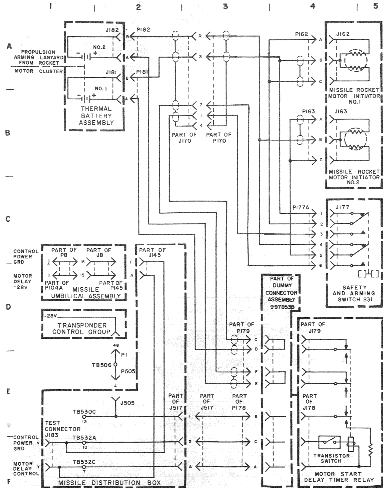
Figure 4-12 (U). Missile propulsion system (U).
