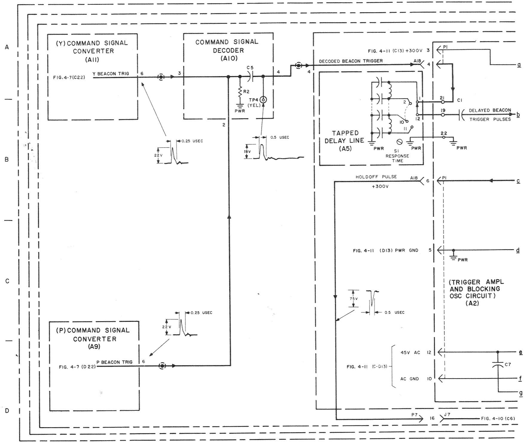
Figure 4-9 (C). Beacon transmitting circuit—functional diagram (mushroom) (sheet 1 of 2) (U).
