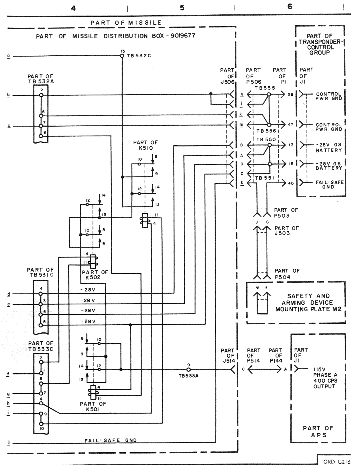
Figure 4-21 (U). Missile guidance set battery, missile reject, and HE prepared circuits—functional diagram (missiles 13684 and subsequent) (sheet 2 of 2) (U).
