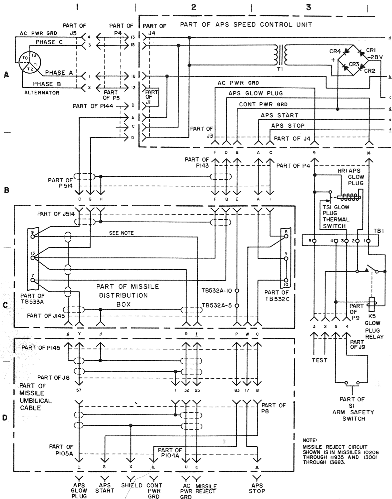
Figure 4-16 (U). Accessory power supply 9030900 electrical control system—functional schematic (serial numbers prior to 69-3632) (sheet 1 of 2) (U).
