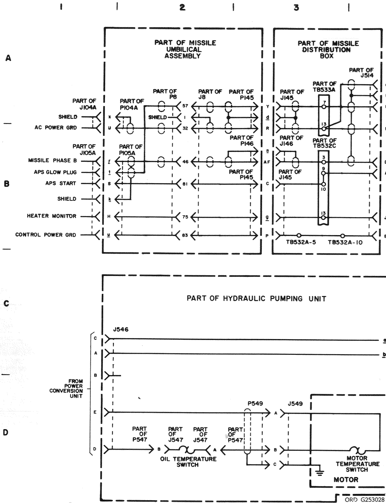
Figure 4-18 (U). Hydraulic pumping unit—functional schematic (sheet 1 of 2) (U).
