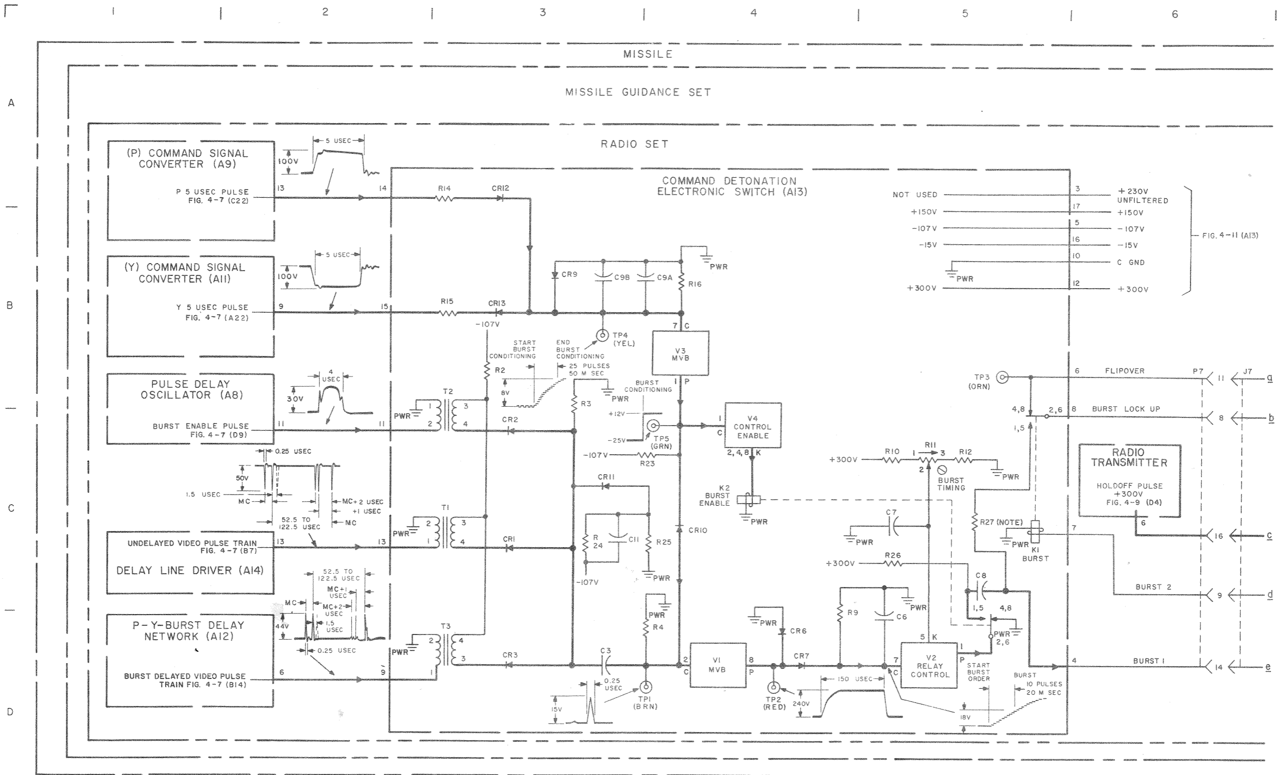
Figure 4-10 (C). Detonation command circuit—functional diagram (mushroom) (sheet 1 of 3) (U).
