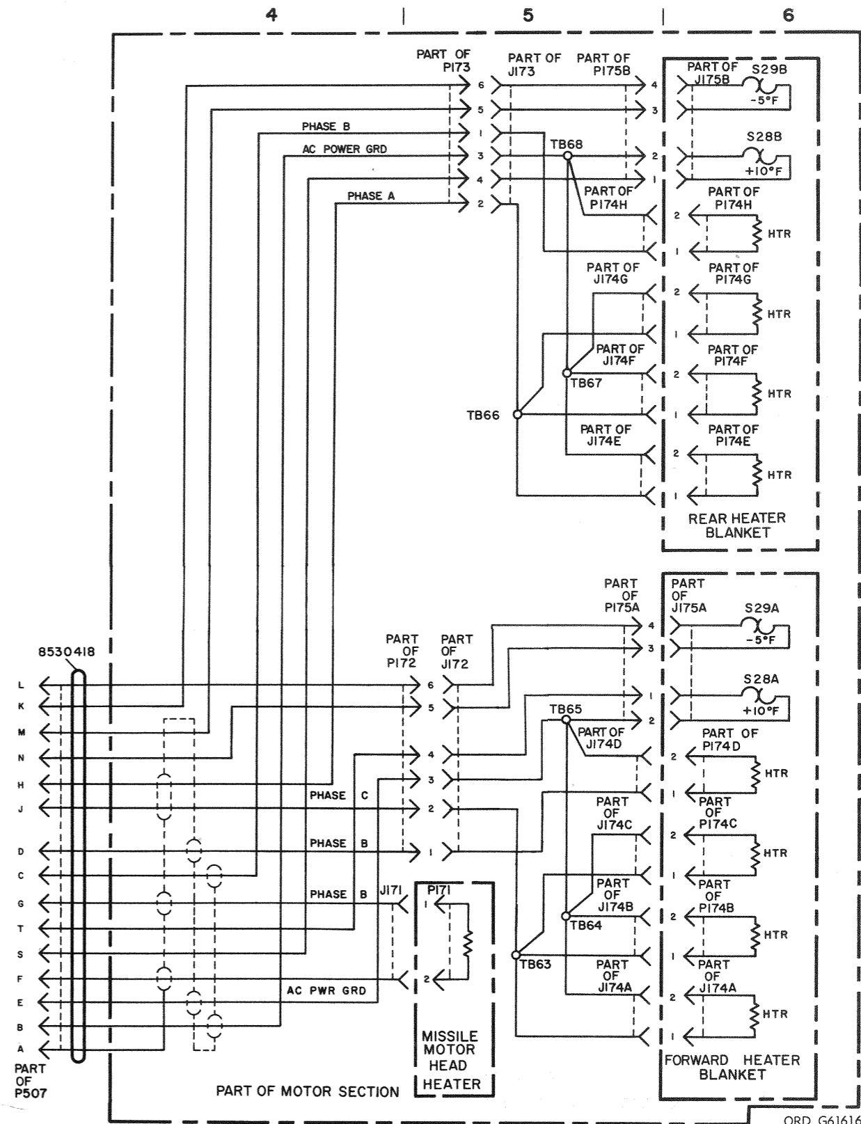
Figure 4-20 (U). Missile heater system—functional diagram (sheet 2 of 2) (U).
