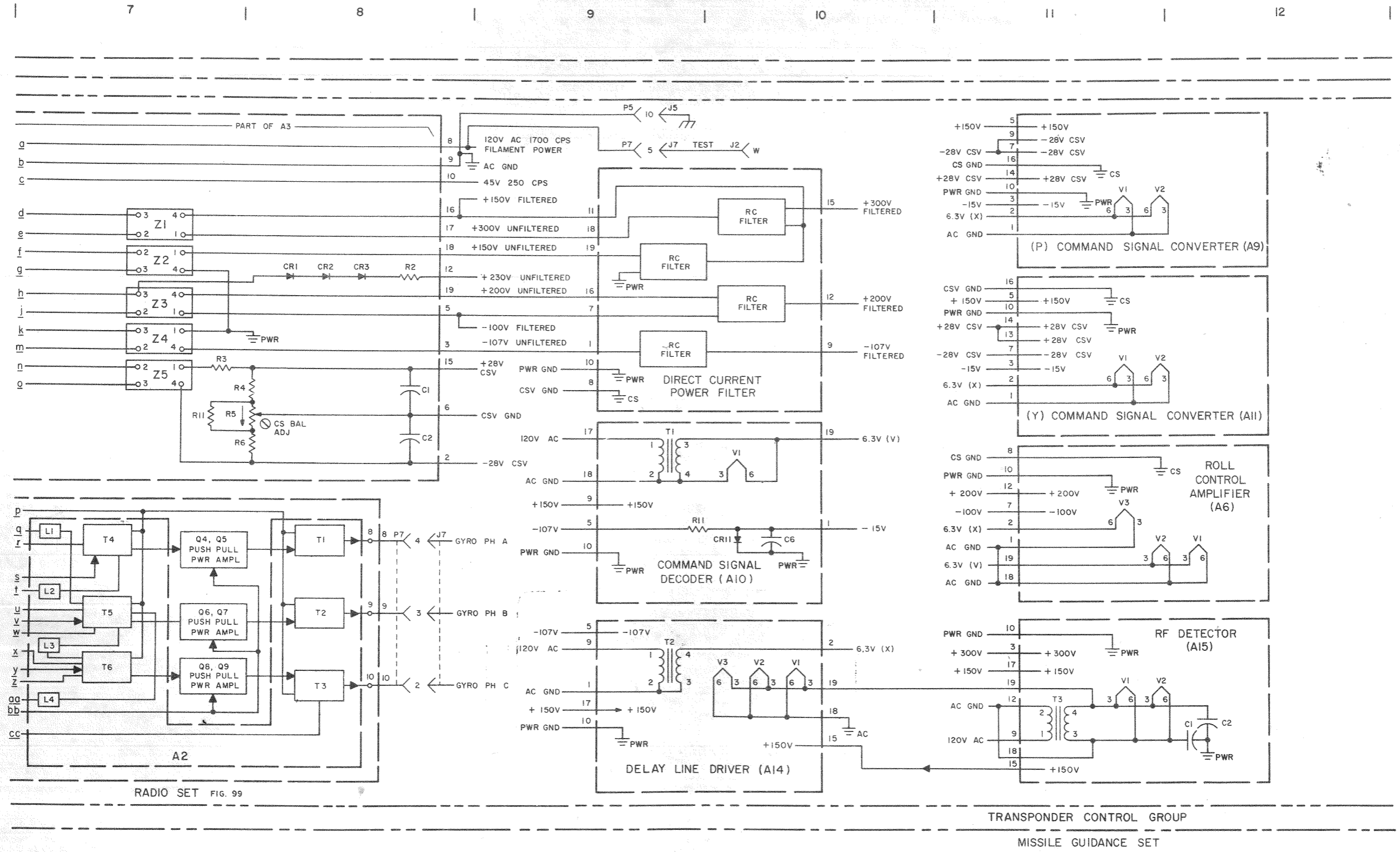
Figure 4-11 (C). Power supply and distribution circuit—functional diagram (mushroom) (sheet 2 of 3) (U).
