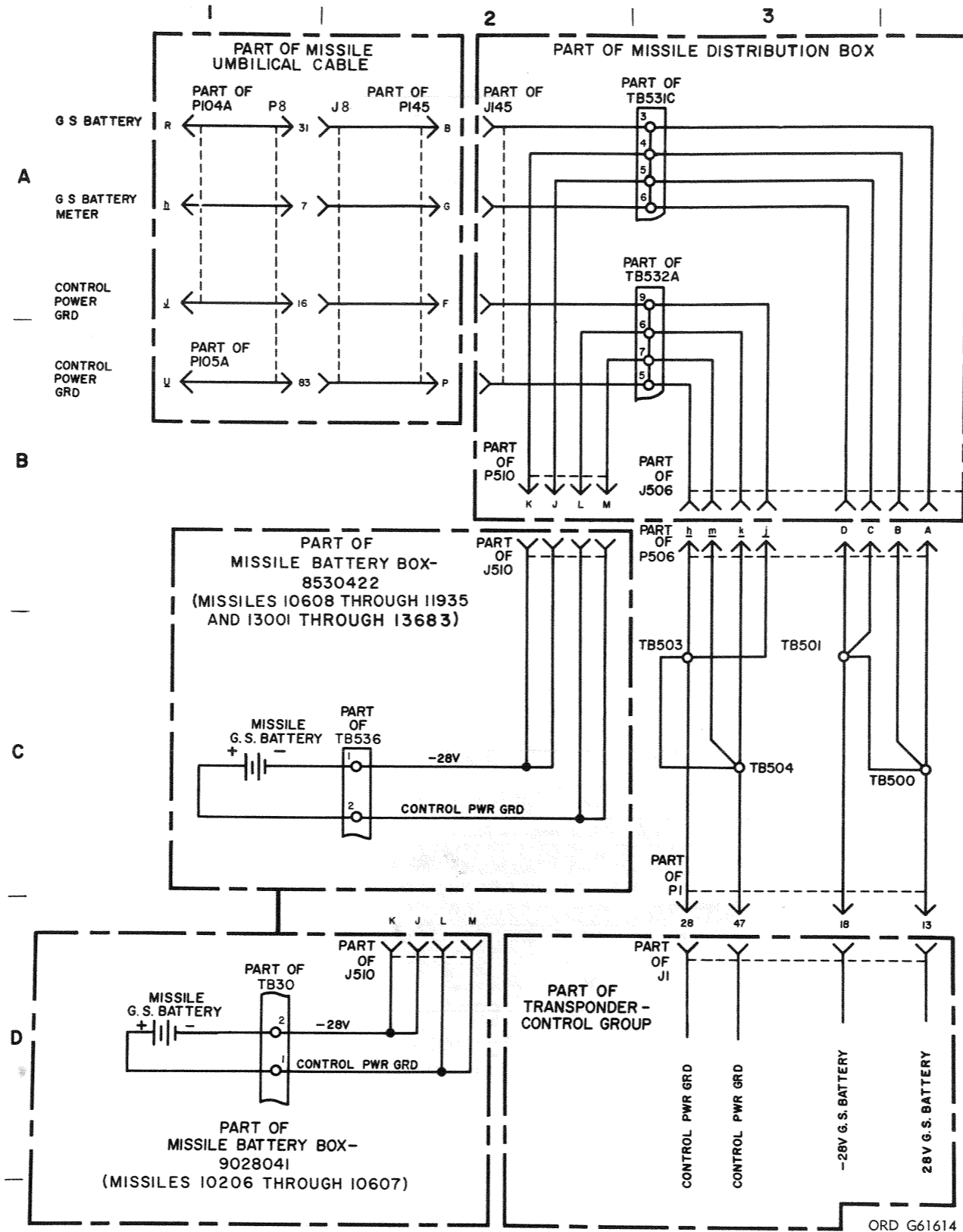
Figure 4-19 (U). Missile guidance set battery—functional schematic (U).
