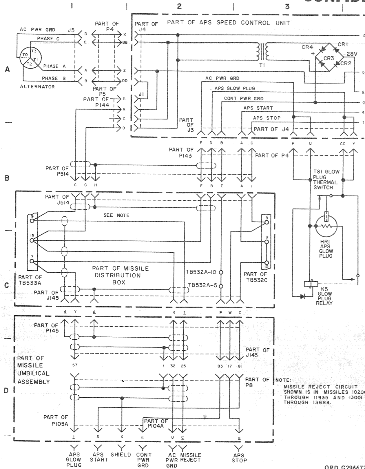
Figure 4-15 (U). Accessory power supply 9032190 electrical control system—functional schematic (sheet 1 of 2) (U).
