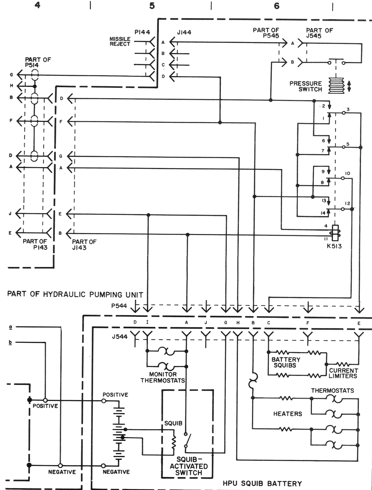
Figure 4-18 (U). Hydraulic pumping unit—functional schematic (sheet 2 of 2) (U).
