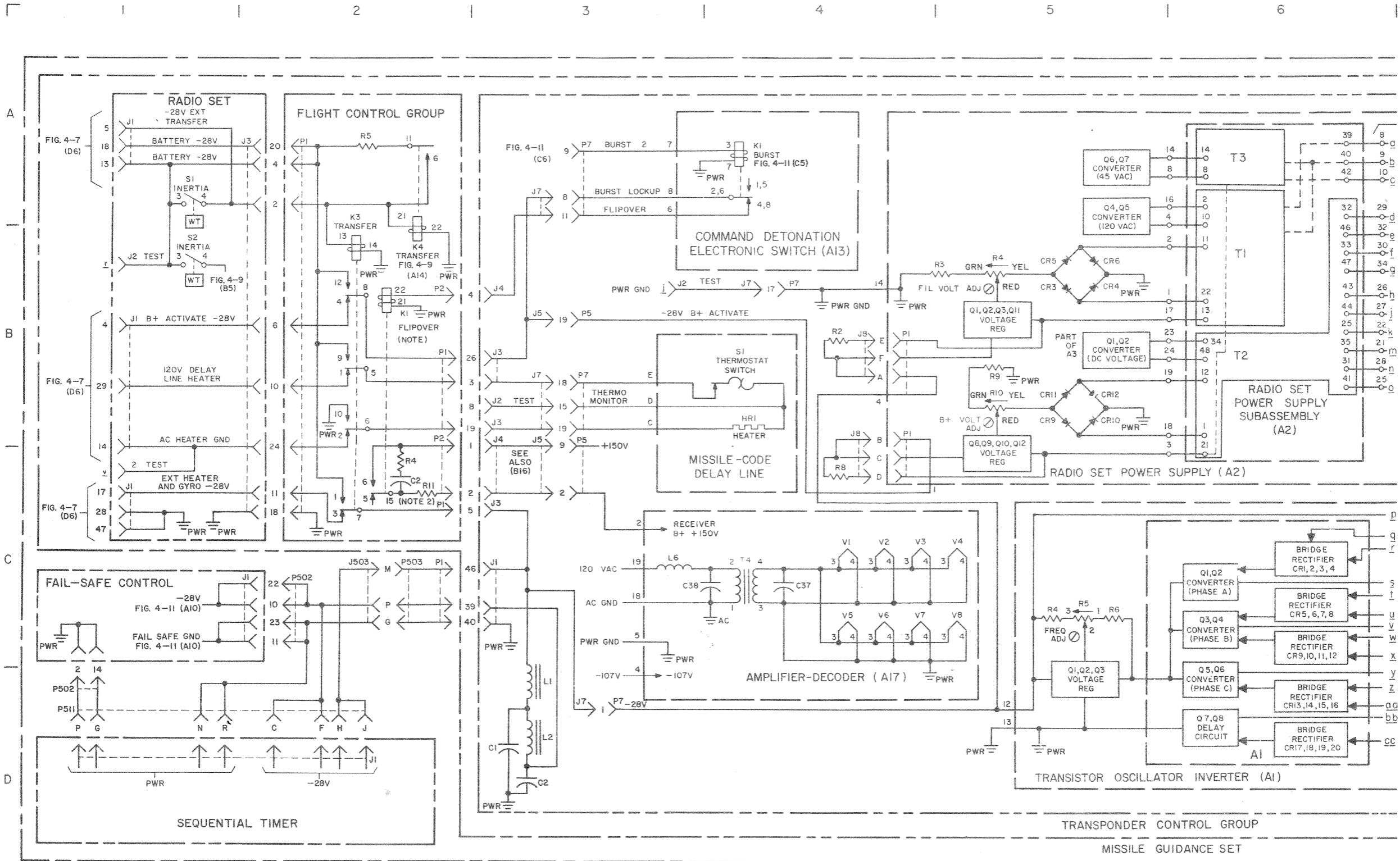
Figure 4-11 (C). Power supply and distribution circuit—functional diagram (mushroom) (sheet 1 of 3) (U).
