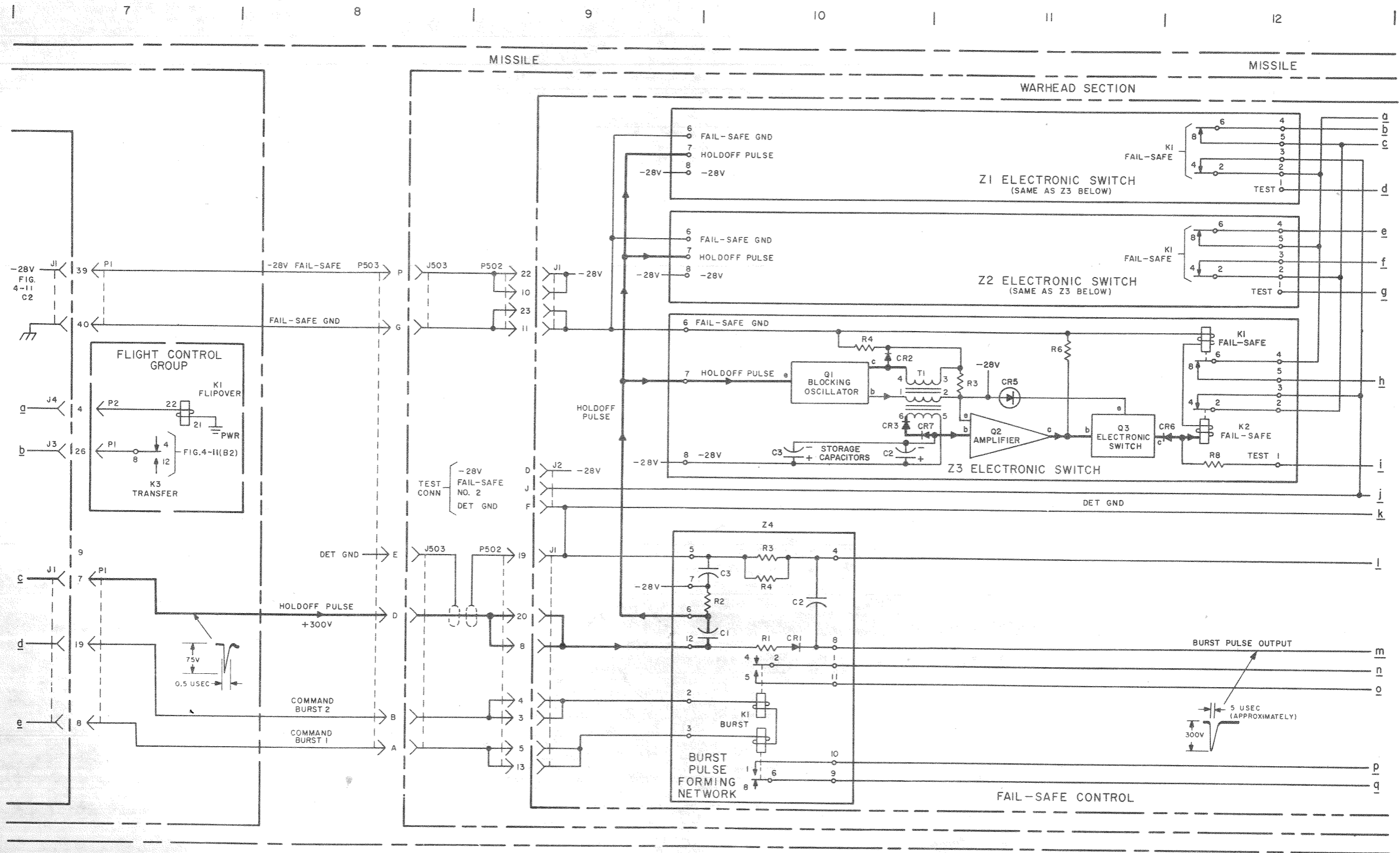
Figure 4-10 (C). Detonation command circuit—functional diagram (mushroom) (sheet 2 of 3) (U).
