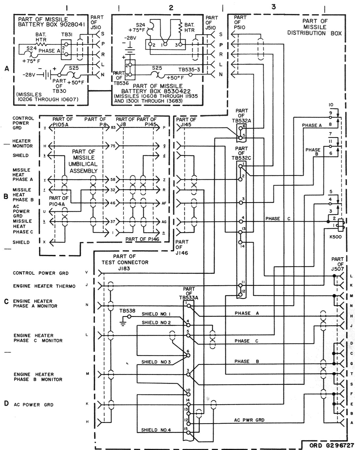
Figure 4-20 (U). Missile heater system—functional diagram (sheet 1 of 2) (U).
