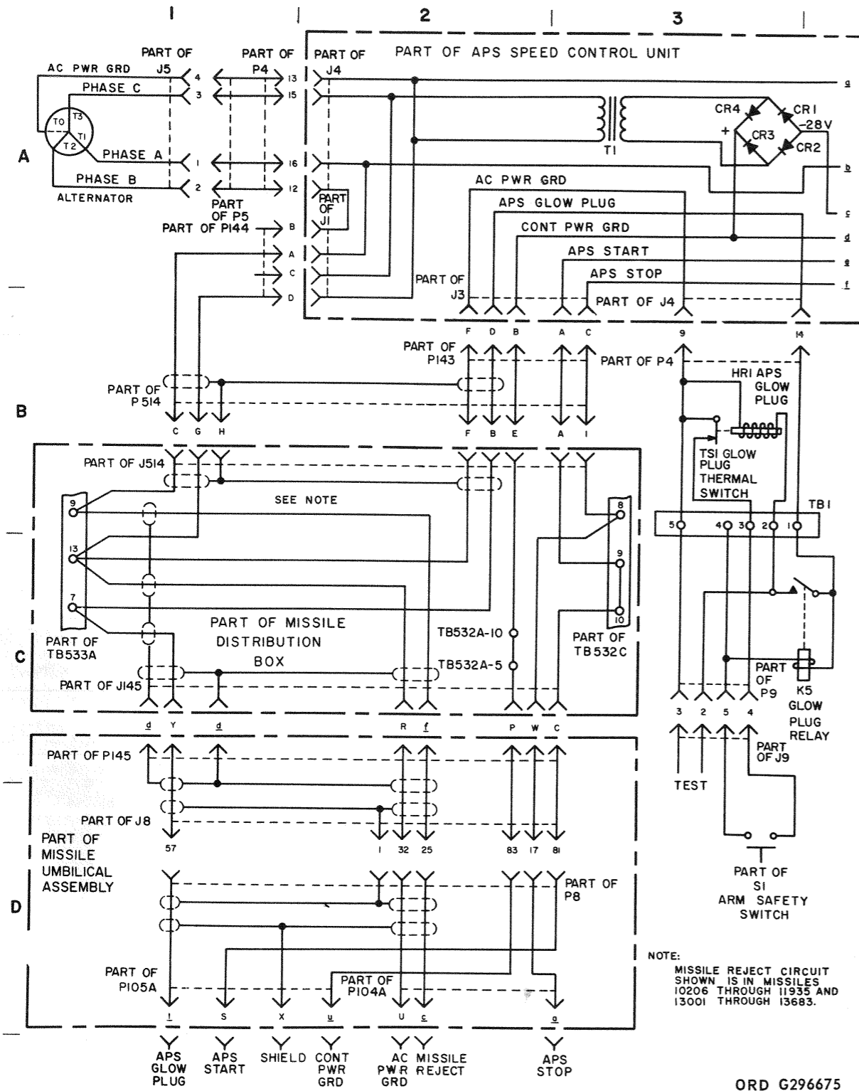
Figure 4-17 (U). Accessory power supply 9030900 electrical control system—functional schematic (serial numbers 69-3632 and subsequent) (sheet 1 of 2) (U).
